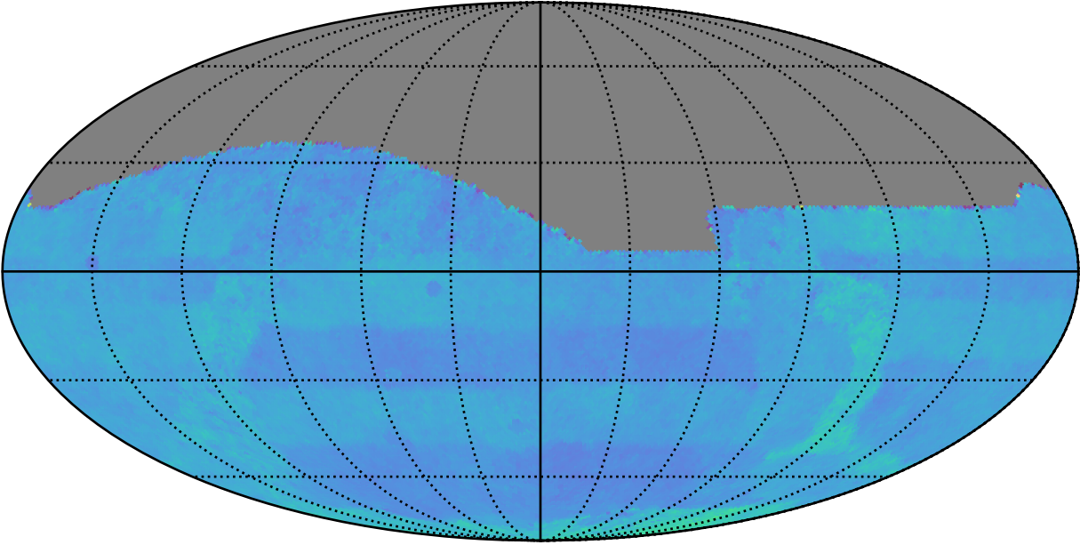
ddf_acor_sf10_lsf20_lsr10_v3.4_10yrs All sky: Normalized Proper Motion Uncert @ 24.0
