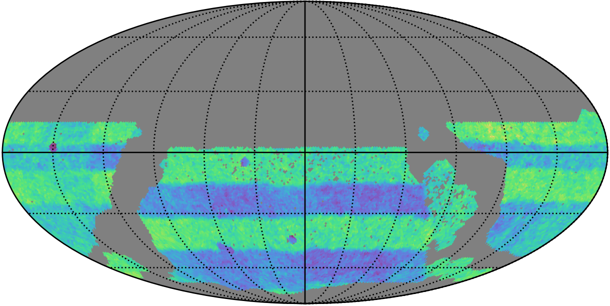
ddf_acor_sf10_lsf20_lsr10_v3.4_10yrs WFD: Normalized Proper Motion Uncert @ 20.5
