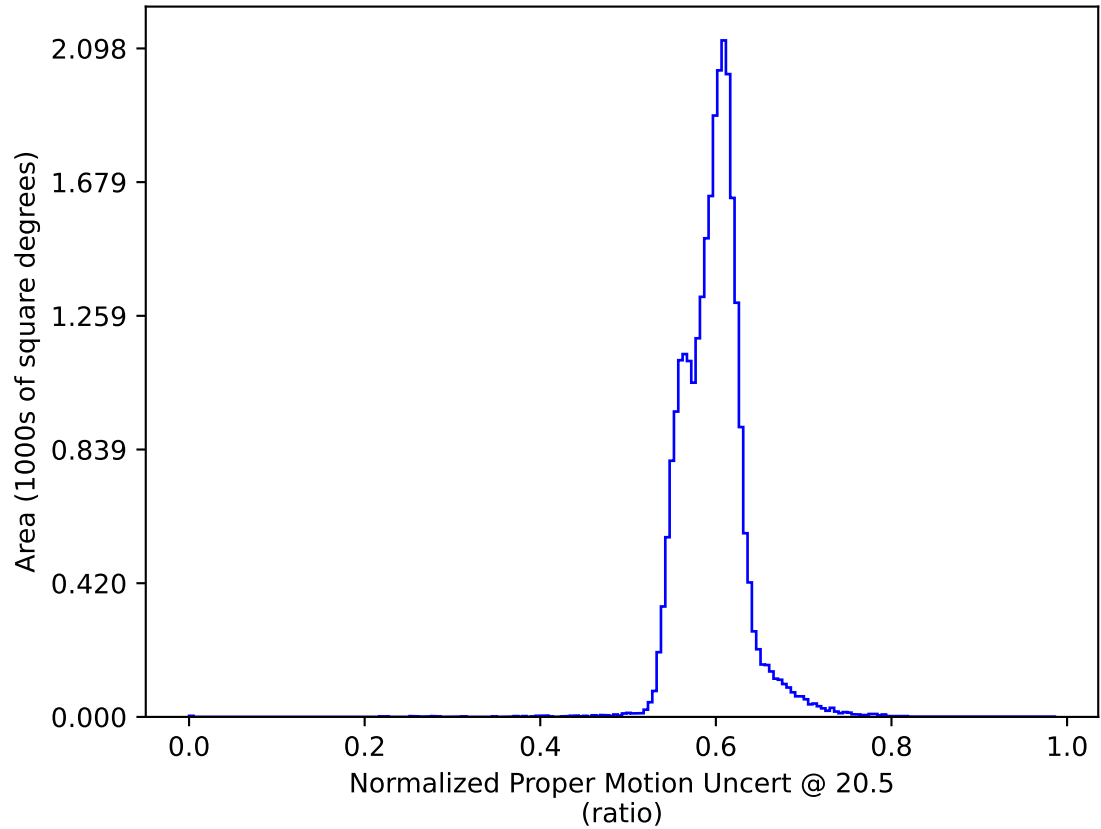
ddf_acor_sf10_lsf20_lsr10_v3.4_10yrs All sky: Normalized Proper Motion Uncert @ 20.5
