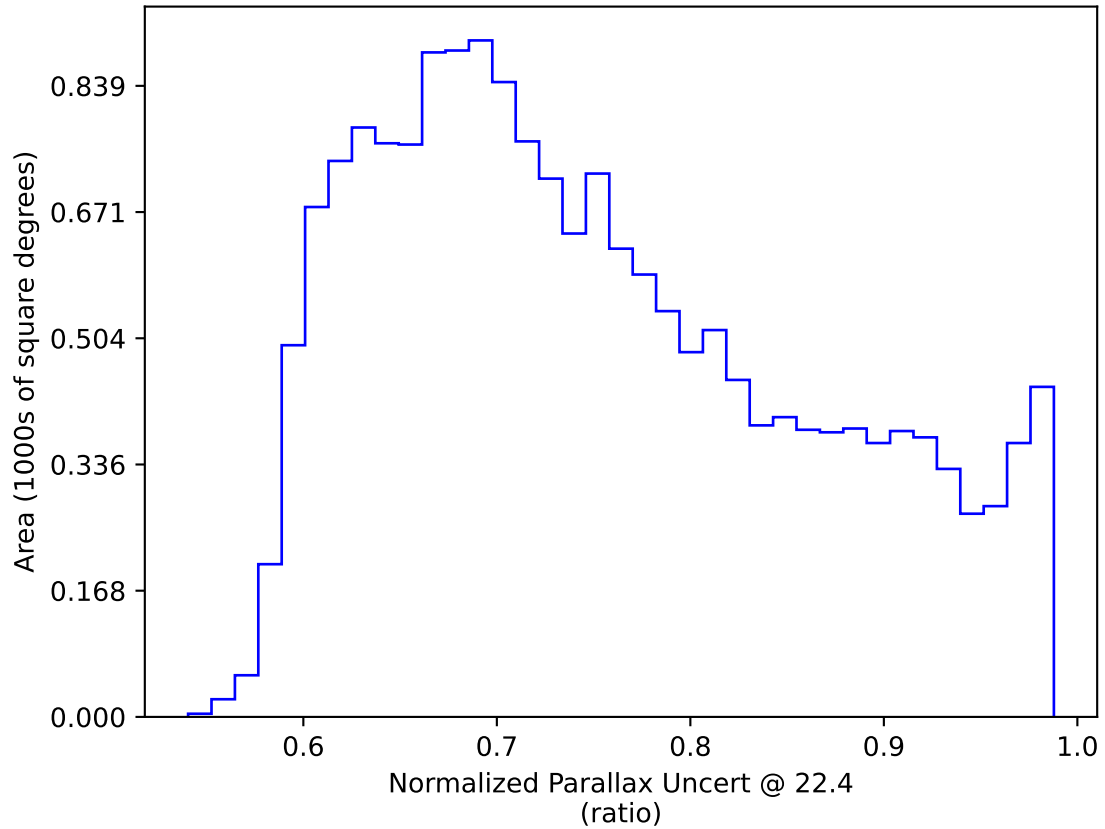
ddf_acor_sf10_ls20_lsr10_v3.4_10yrs WFD: Normalized Parallax Uncert @ 22.4
