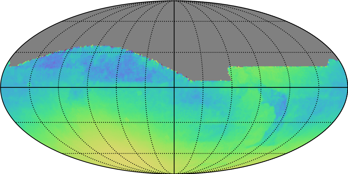
ddf_acor_sf10_lsf20_lsr10_v3.4_10yrs All sky: Normalized Parallax Uncert @ 22.4
