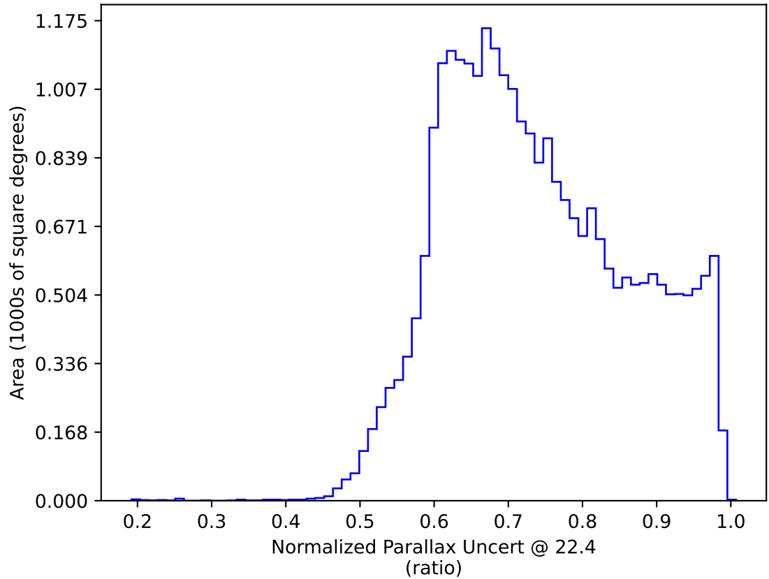
ddf_acor_sf10_lsf20_lsr10_v3.4_10yrs All sky: Normalized Parallax Uncert @ 22.4
