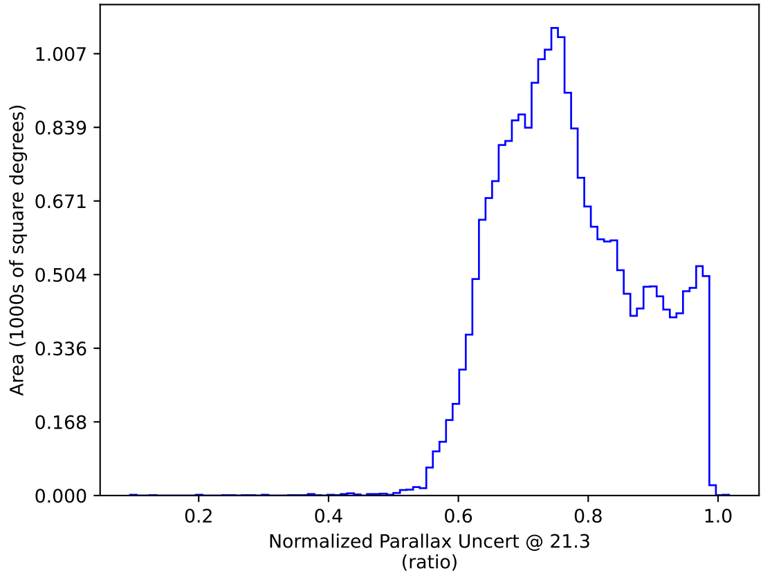
ddf_acor_sf10_lsf20_lsr10_v3.4_10yrs All sky y band only: Normalized Parallax Uncert @ 21.3
