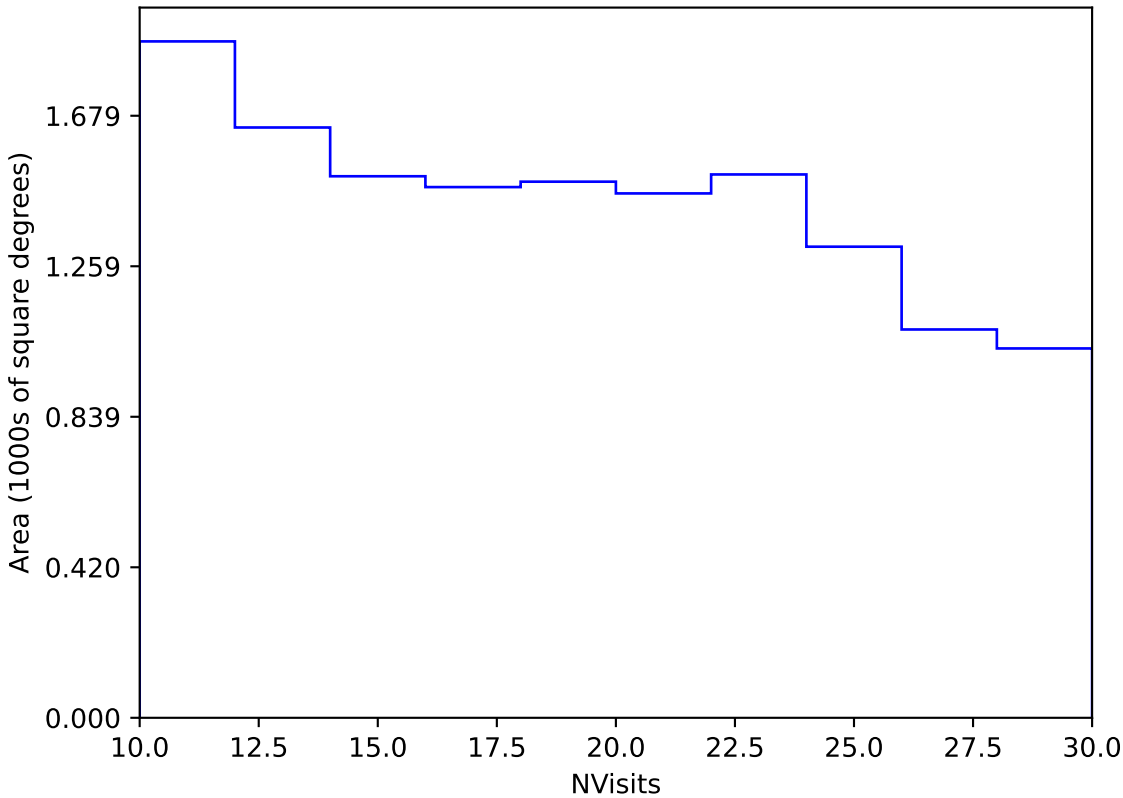
ddf_acor_sf10_lsf20_lsr10_v3.4_10yrs Yr 3-4 y band: NVisits
