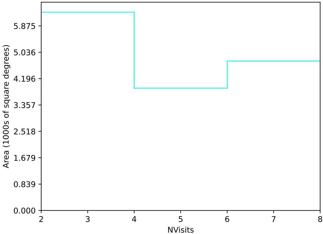
ddf_acor_sf10_lsf20_lsr10_v3.4_10yrs Yr 3-4 u band: NVisits
