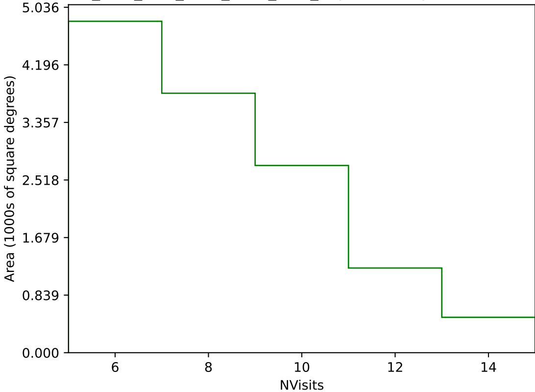
ddf_acor_sf10_lsf20_lsr10_v3.4_10yrs Yr 3-4 g band: NVisits
