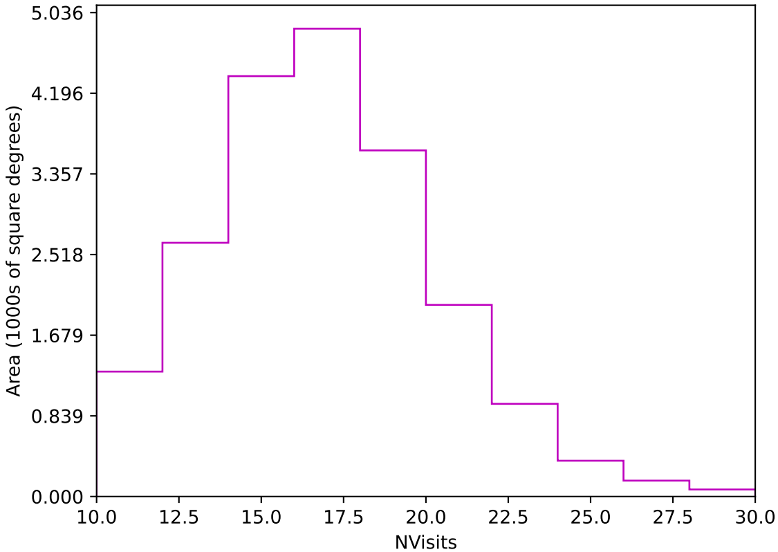
ddf_acor_sf10_lsf20_lsr10_v3.4_10yrs Yr 1 z band: NVisits
