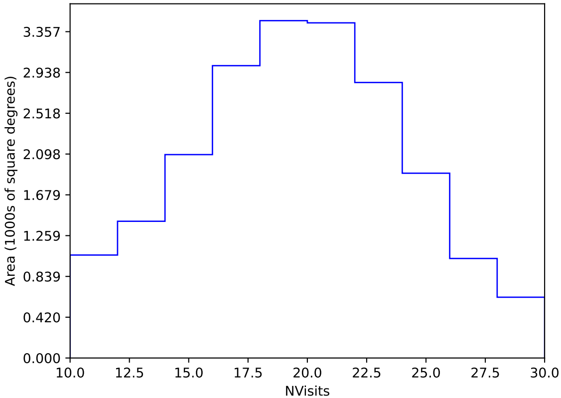
ddf_acor_sf10_lsf20_lsr10_v3.4_10yrs Yr 1 y band: NVisits
