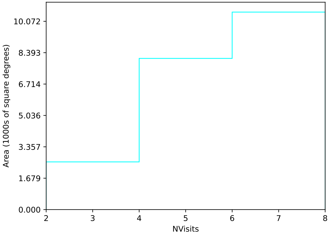
ddf_acor_sf10_lsf20_lsr10_v3.4_10yrs Yr 1 u band: NVisits
