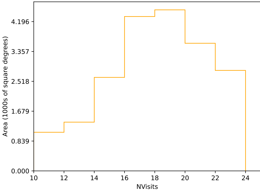
ddf_acor_sf10_lsf20_lsr10_v3.4_10yrs Yr 1 r band: NVisits
