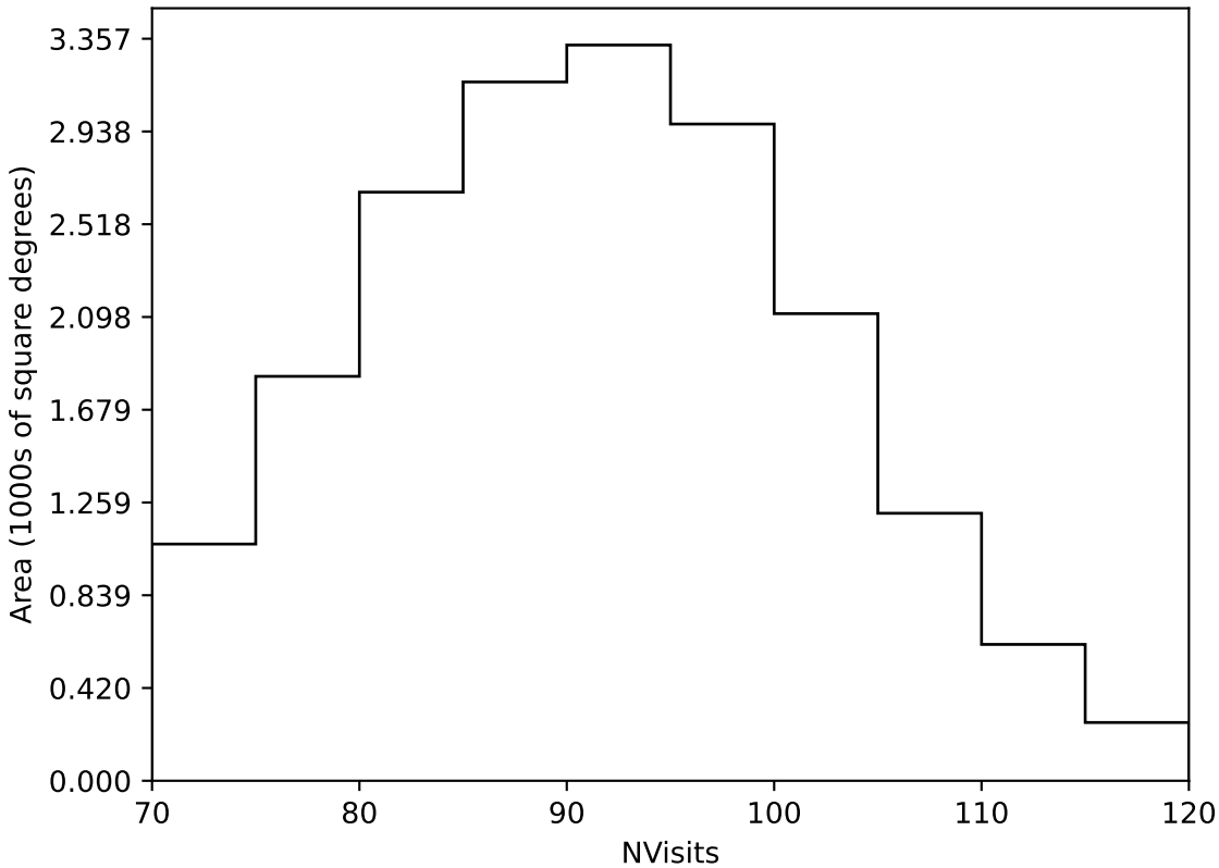
ddf_acor_sf10_lsf20_lsr10_v3.4_10yrs Yr 1 all bands: NVisits
