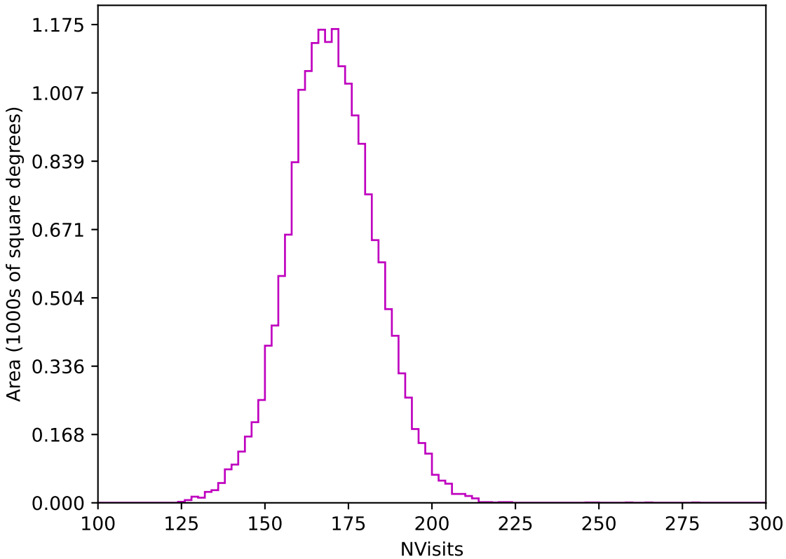
ddf_acor_sf10_lsf20_lsr10_v3.4_10yrs WFD z band: NVisits
