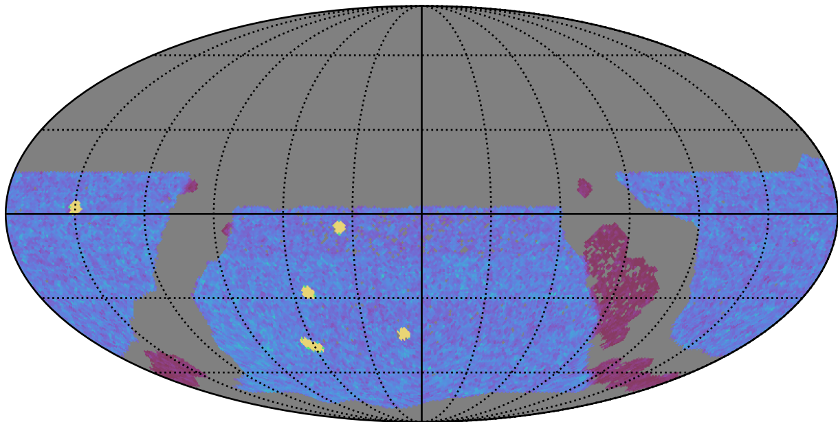
ddf_acor_sf10_lsf20_lsr10_v3.4_10yrs WFD y band: NVisits
