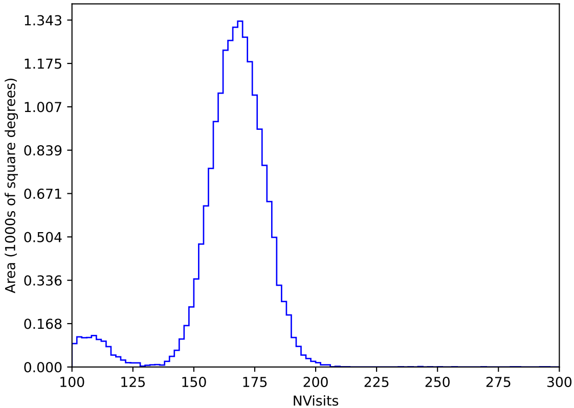
ddf_acor_sf10_lsf20_lsr10_v3.4_10yrs WFD y band: NVisits
