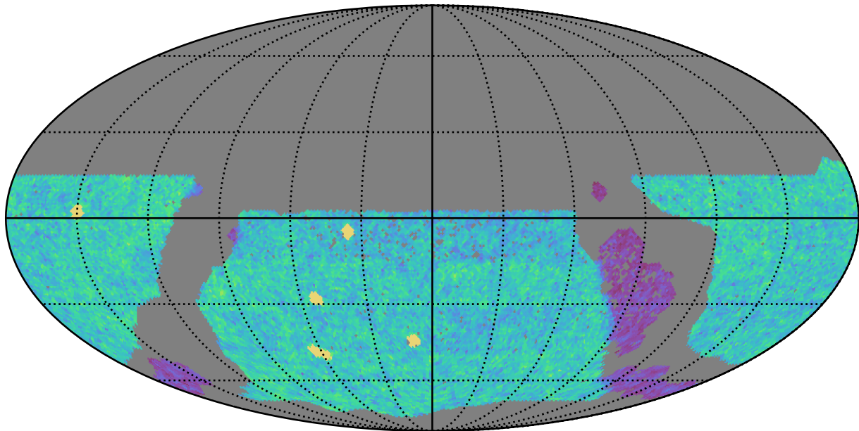
ddf_acor_sf10_lsf20_lsr10_v3.4_10yrs WFD u band: NVisits
