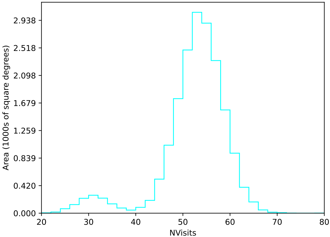
ddf_acor_sf10_lsf20_lsr10_v3.4_10yrs WFD u band: NVisits
