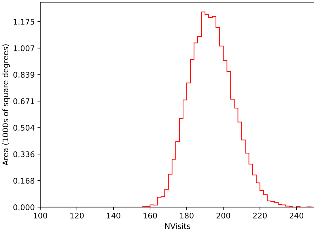
ddf_acor_sf10_lsf20_lsr10_v3.4_10yrs WFD i band: NVisits
