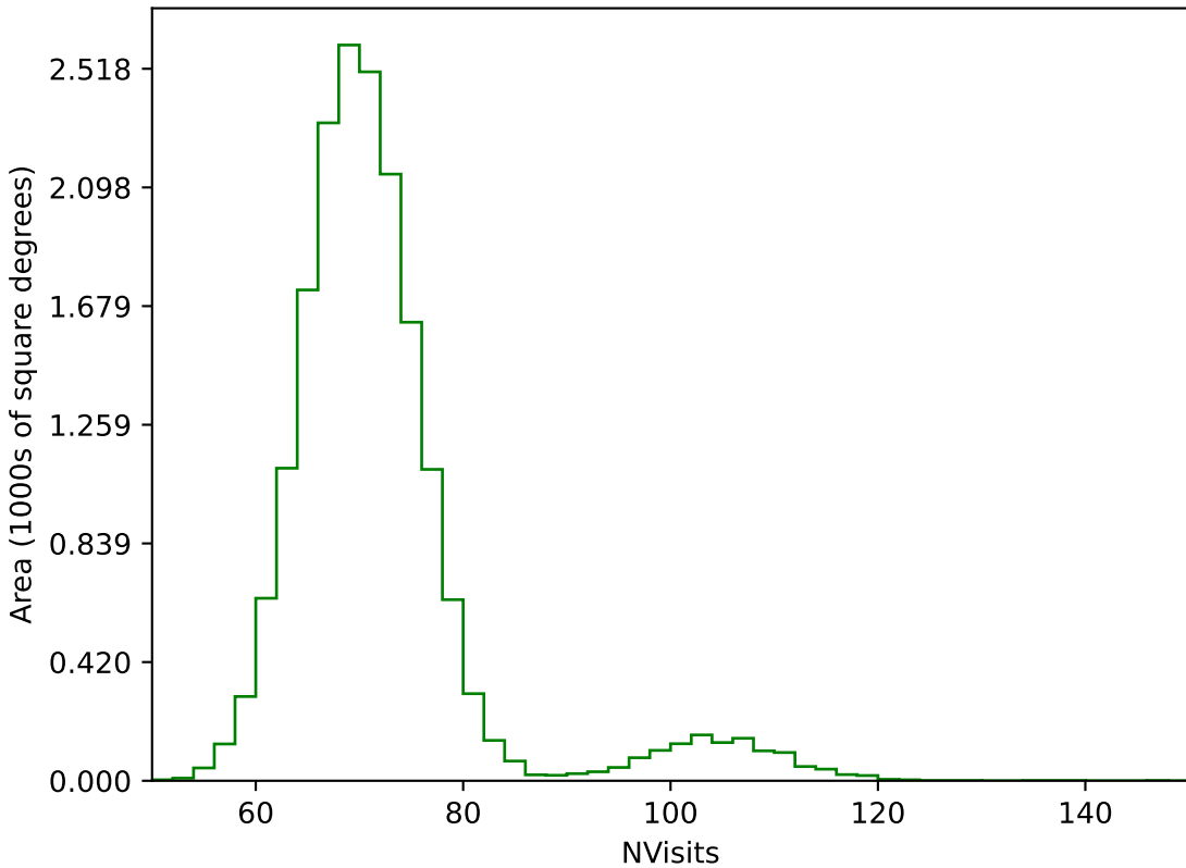
ddf_acor_sf10_lsf20_lsr10_v3.4_10yrs WFD g band: NVisits
