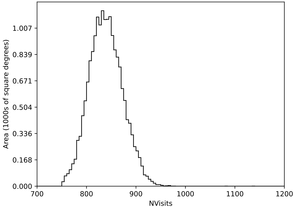
ddf_acor_sf10_lsf20_lsr10_v3.4_10yrs WFD all bands: NVisits
