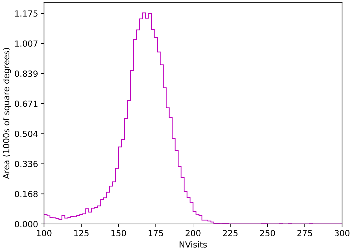
ddf_acor_sf10_lsf20_lsr10_v3.4_10yrs All sky z band: NVisits
