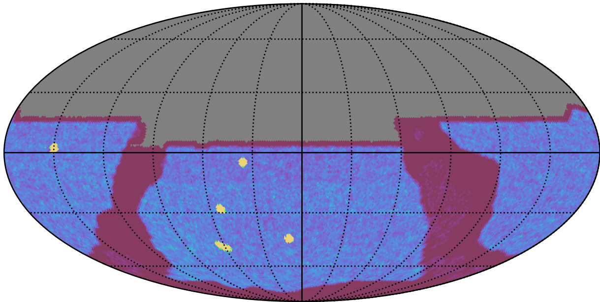
ddf_acor_sf10_lsf20_lsr10_v3.4_10yrs All sky y band: NVisits
