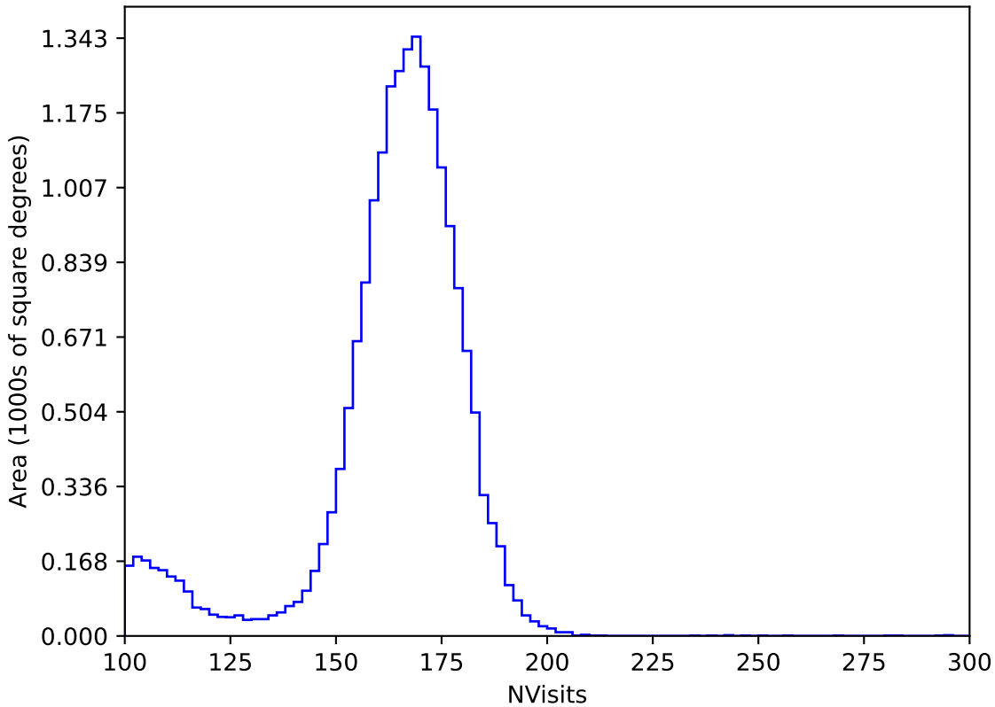
ddf_acor_sf10_lsf20_lsr10_v3.4_10yrs All sky y band: NVisits
