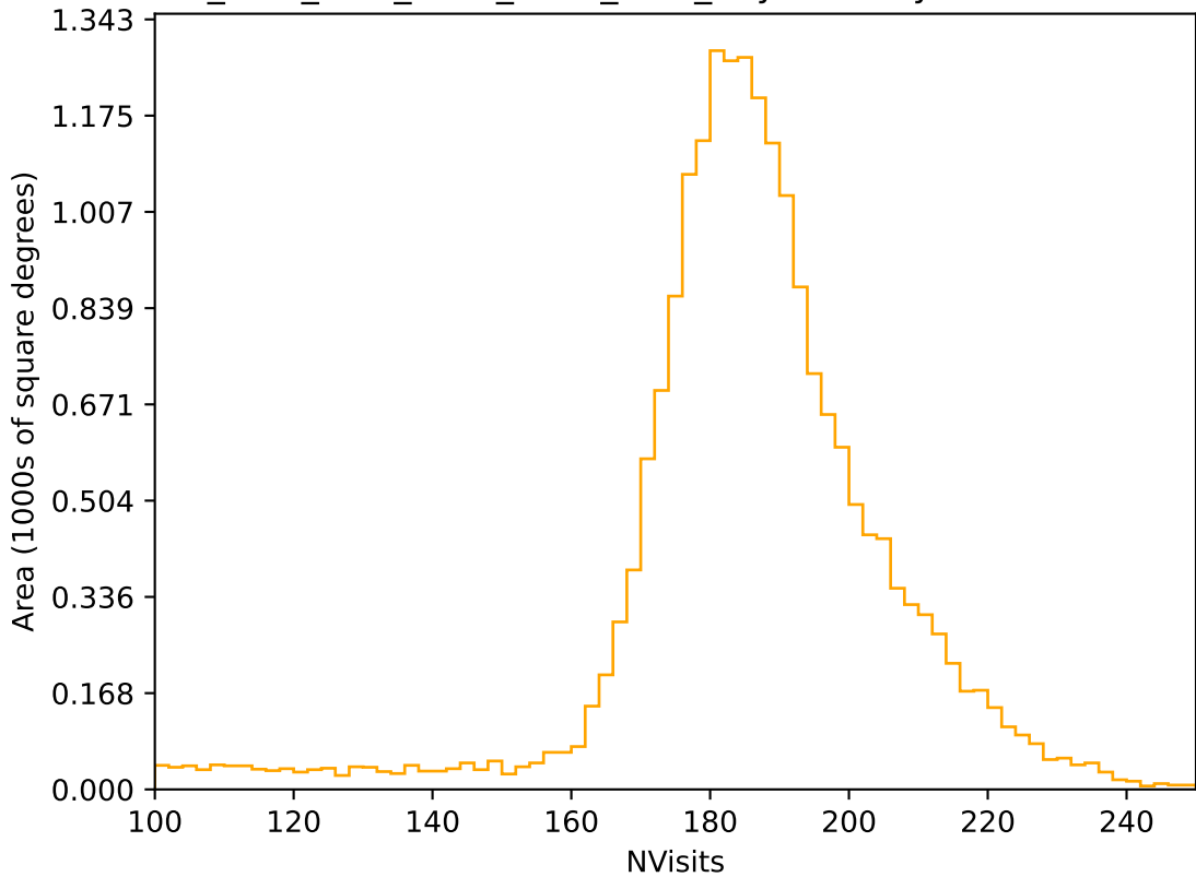
ddf_acor_sf10_lsf20_lsr10_v3.4_10yrs All sky r band: NVisits
