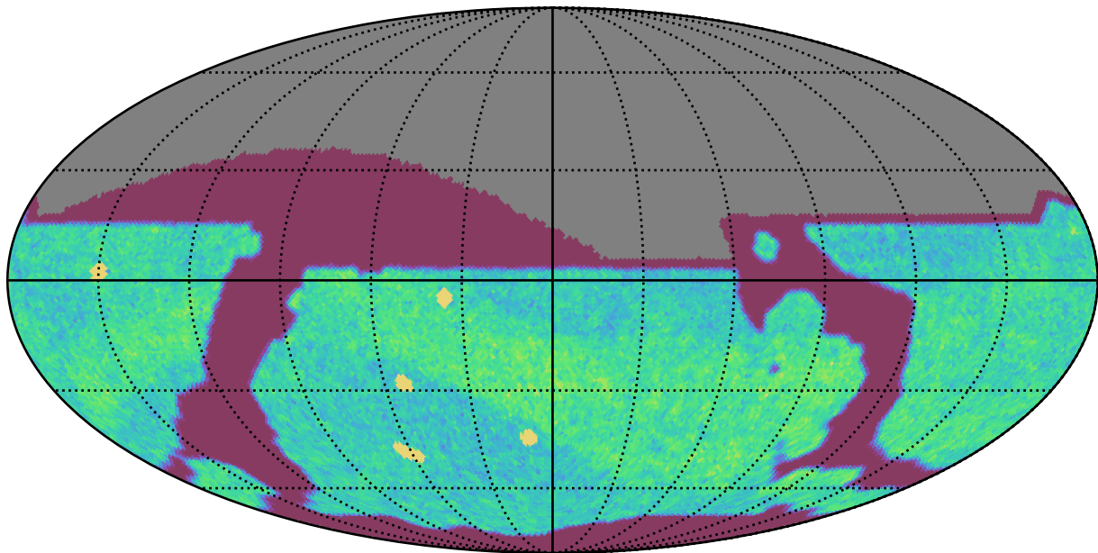
ddf_acor_sf10_lsf20_lsr10_v3.4_10yrs All sky i band: NVisits
