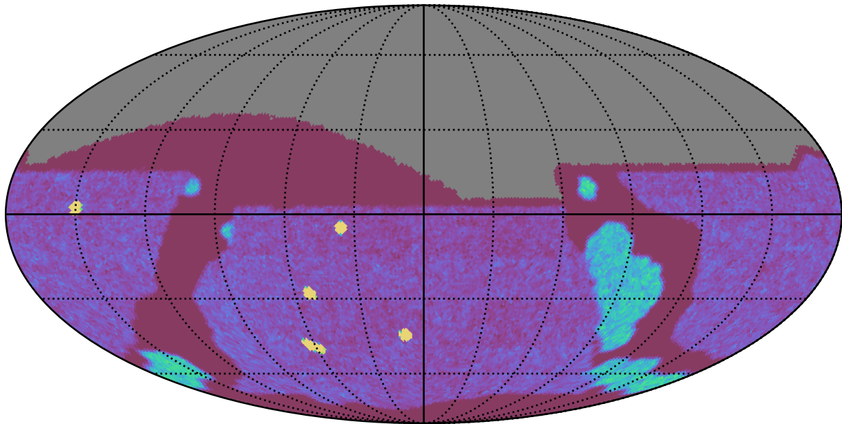
ddf_acor_sf10_lsf20_lsr10_v3.4_10yrs All sky g band: NVisits
