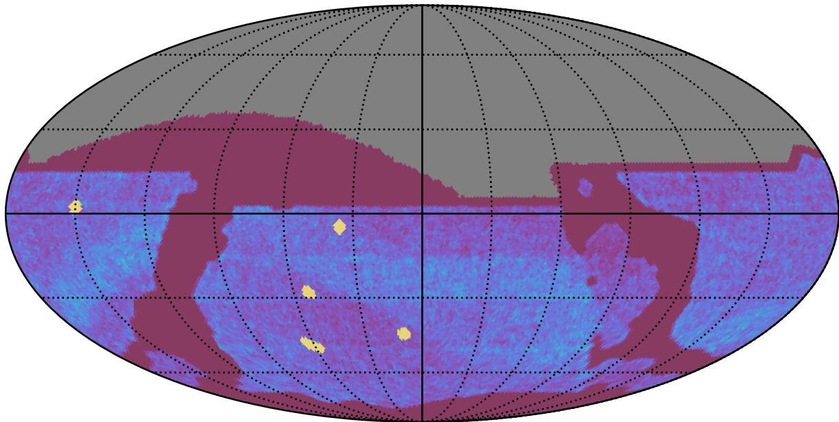
ddf_acor_sf10_lsf20_lsr10_v3.4_10yrs All sky all bands: NVisits
