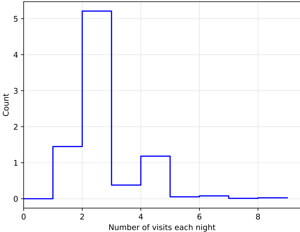
ddf_acor_sf10_lsf20_lsr10_v3.4_10yrs WFD: NVisitsPerNight 1e6
