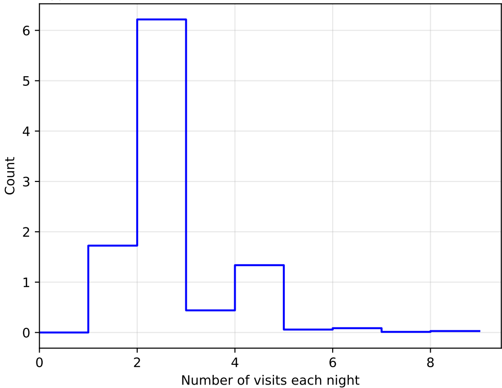
ddf_acor_sf10_lsf20_lsr10_v3.4_10yrs All sky: NVisitsPerNight 1e6
