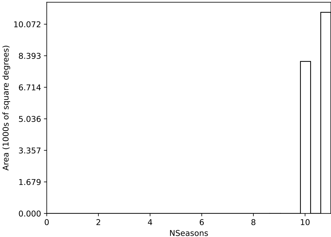
ddf_acor_sf10_lsf20_lsr10_v3.4_10yrs WFD all bands: NSeasons
