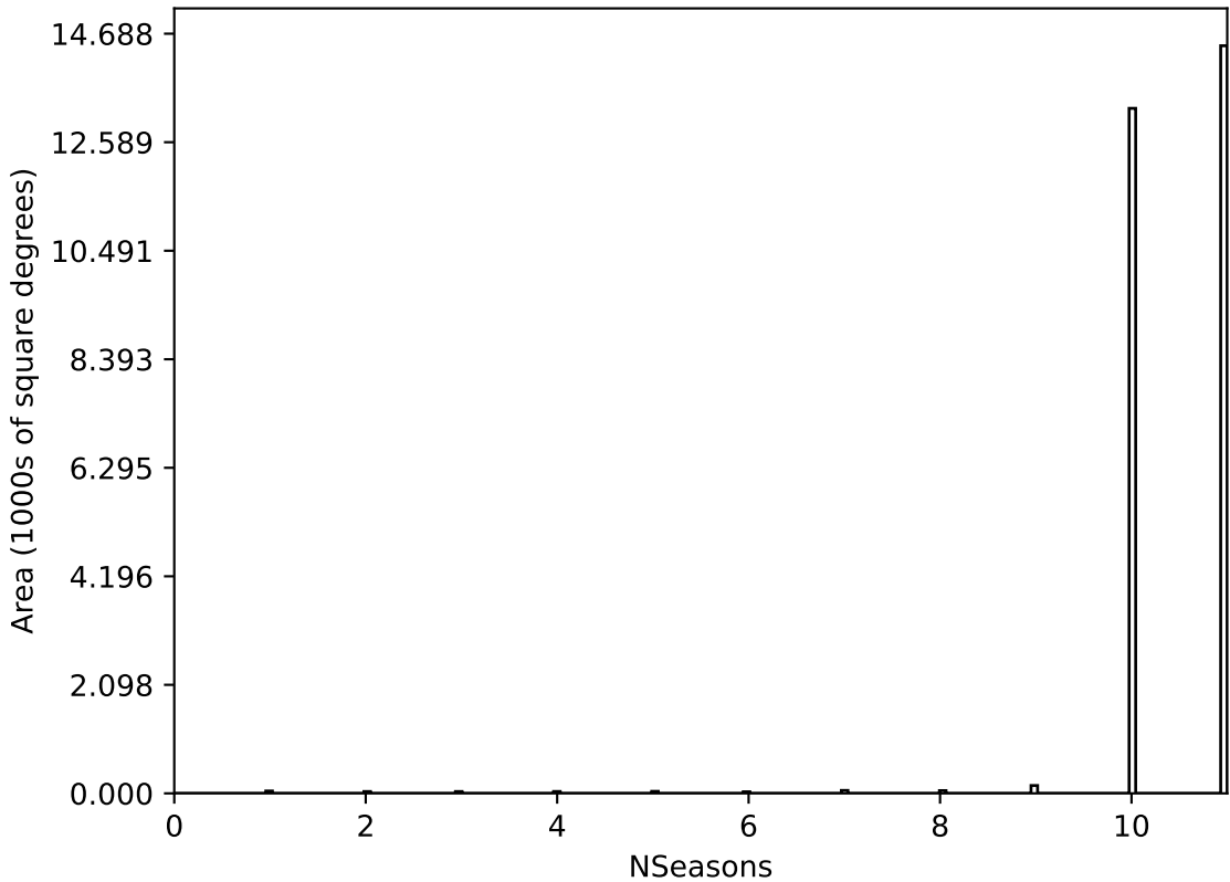
ddf_acor_sf10_lsf20_lsr10_v3.4_10yrs All sky all bands: NSeasons
