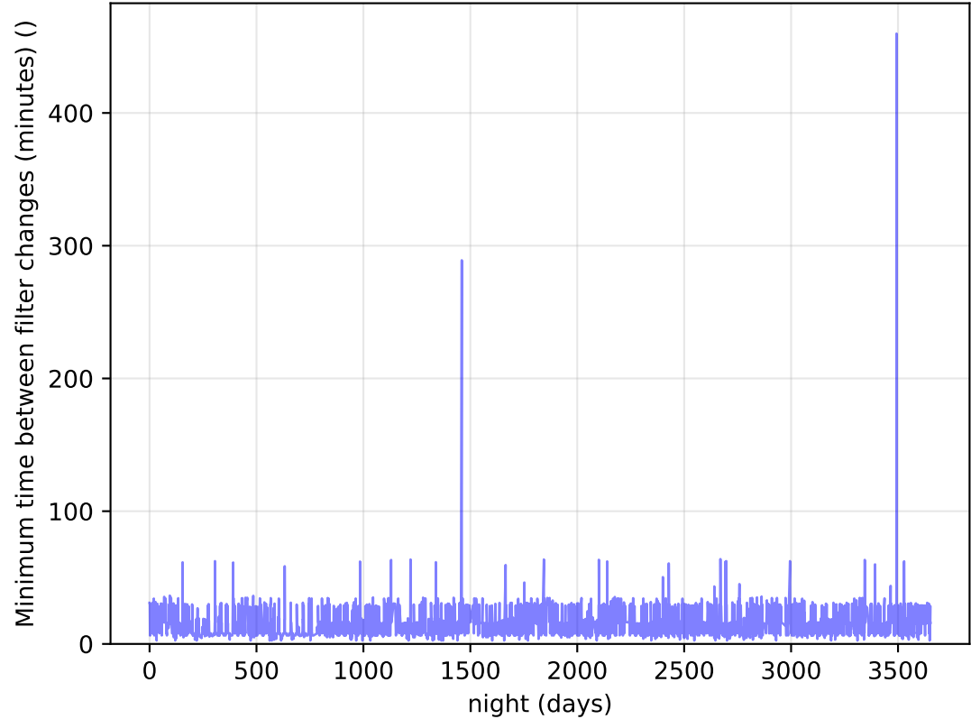
ddf_acor_sf10_Isf20_Isr10_v3.4_10yrs Per Night: Minimum time between filter changes (minutes)
