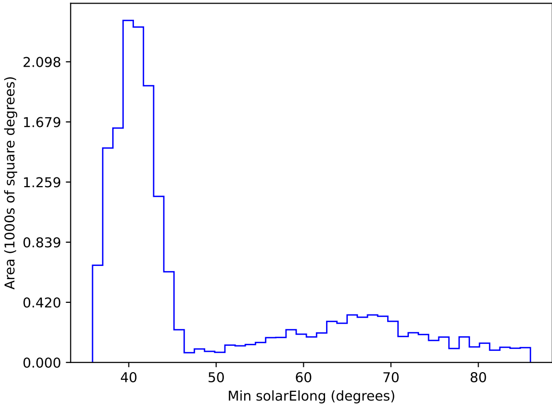
ddf_acor_sf10_lsf20_lsr10_v3.4_10yrs WFD z band: Min solarElong
