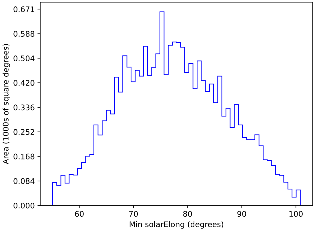
ddf_acor_sf10_lsf20_lsr10_v3.4_10yrs WFD u band: Min solarElong
