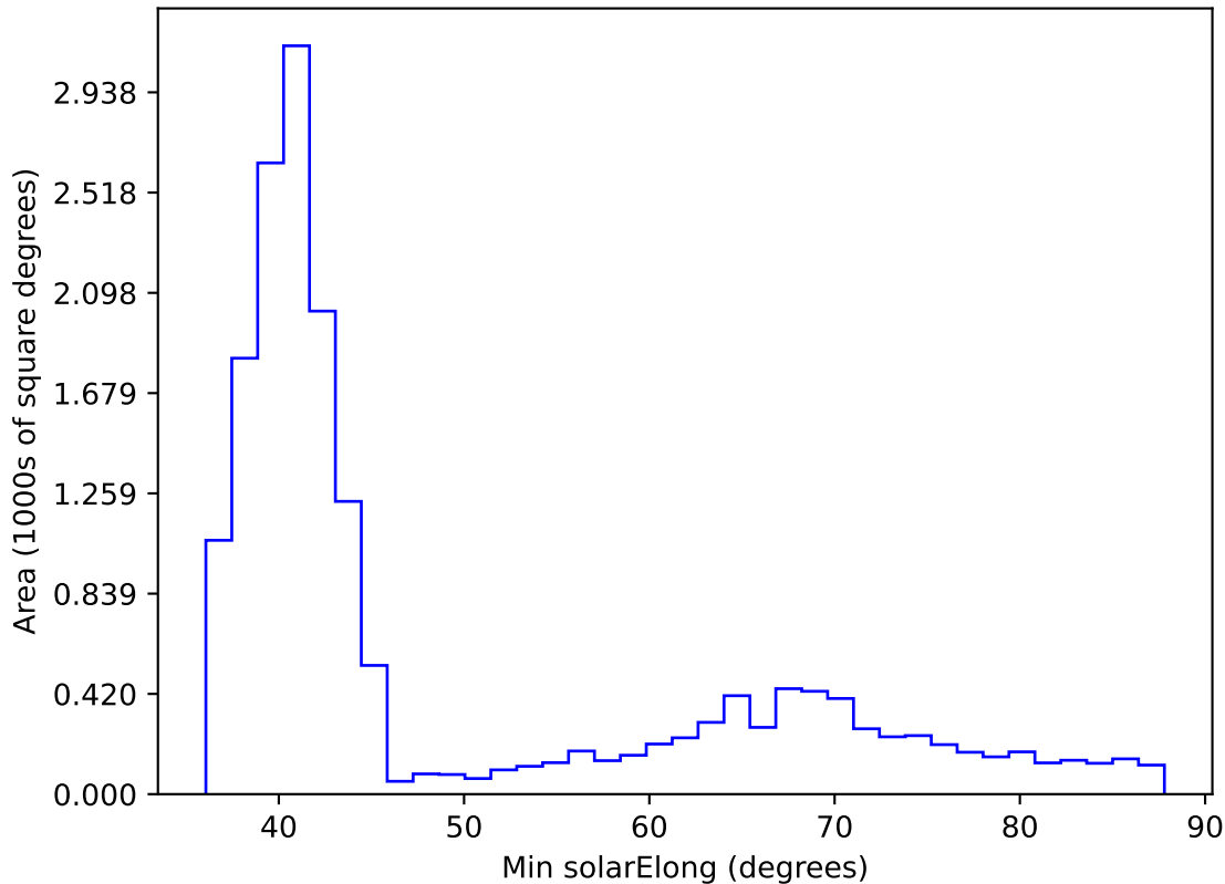
ddf_acor_sf10_lsf20_lsr10_v3.4_10yrs WFD i band: Min solarElong
