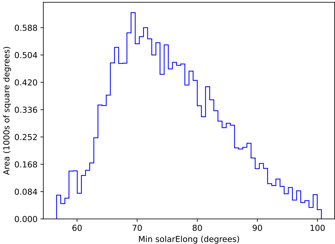
ddf_acor_sf10_lsf20_lsr10_v3.4_10yrs WFD g band: Min solarElong
