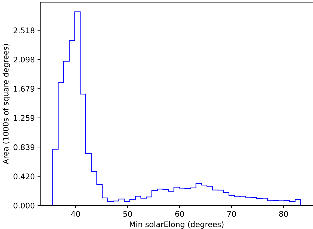
ddf_acor_sf10_lsf20_lsr10_v3.4_10yrs WFD all bands: Min solarElong
