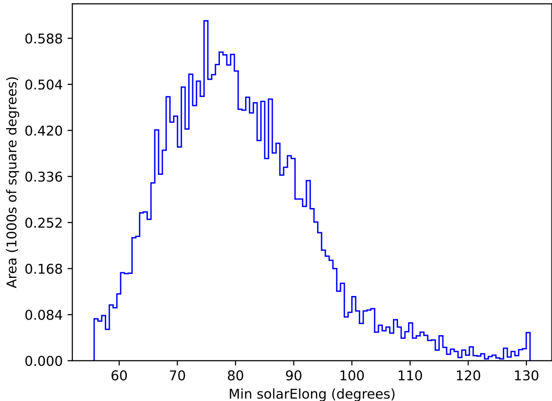
ddf_acor_sf10_lsf20_lsr10_v3.4_10yrs All sky u band: Min solarElong
