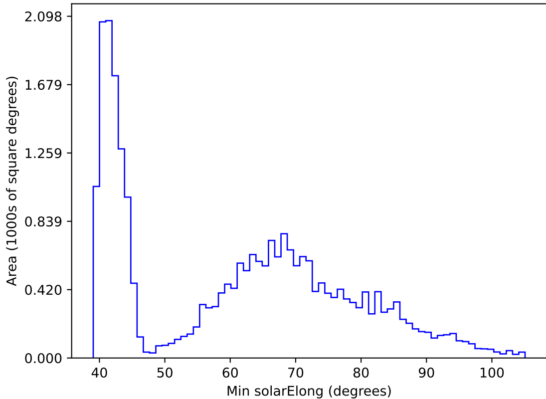
ddf_acor_sf10_lsf20_lsr10_v3.4_10yrs All sky r band: Min solarElong
