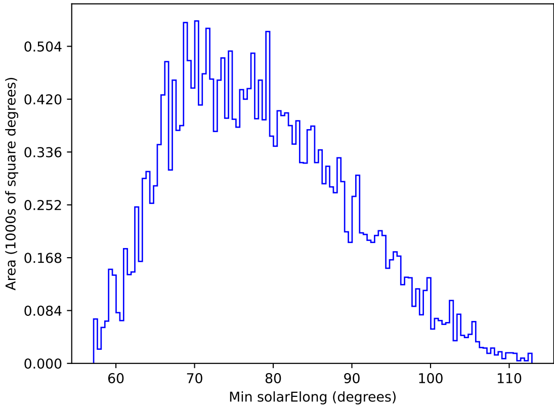
ddf_acor_sf10_lsf20_lsr10_v3.4_10yrs All sky g band: Min solarElong
