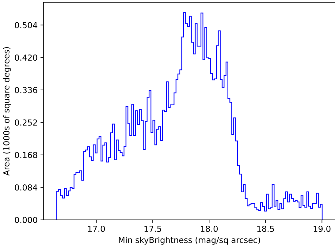
ddf_acor_sf10_lsf20_lsr10_v3.4_10yrs Yr 1 all bands: Min skyBrightness
