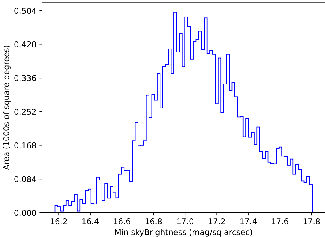
ddf_acor_sf10_lsf20_lsr10_v3.4_10yrs WFD y band: Min skyBrightness
