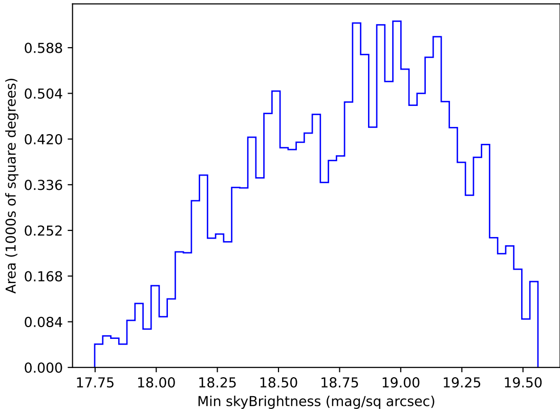
ddf_acor_sf10_lsf20_lsr10_v3.4_10yrs WFD r band: Min skyBrightness
