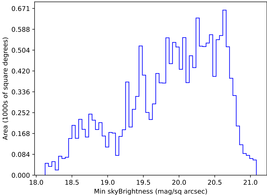
ddf_acor_sf10_lsf20_lsr10_v3.4_10yrs WFD g band: Min skyBrightness
