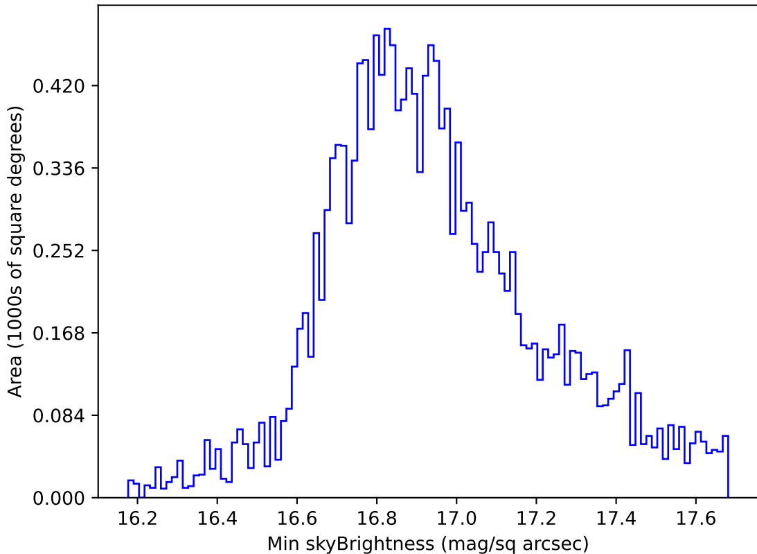
ddf_acor_sf10_lsf20_lsr10_v3.4_10yrs WFD all bands: Min skyBrightness
