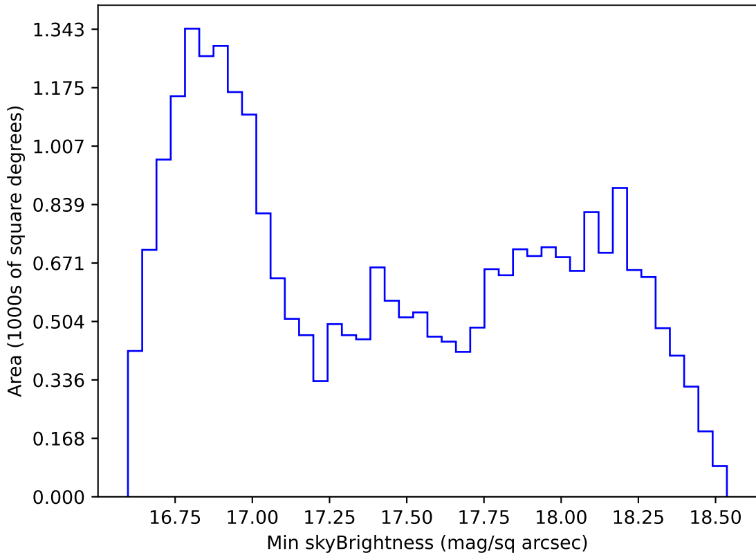
ddf_acor_sf10_lsf20_lsr10_v3.4_10yrs All sky z band: Min skyBrightness
