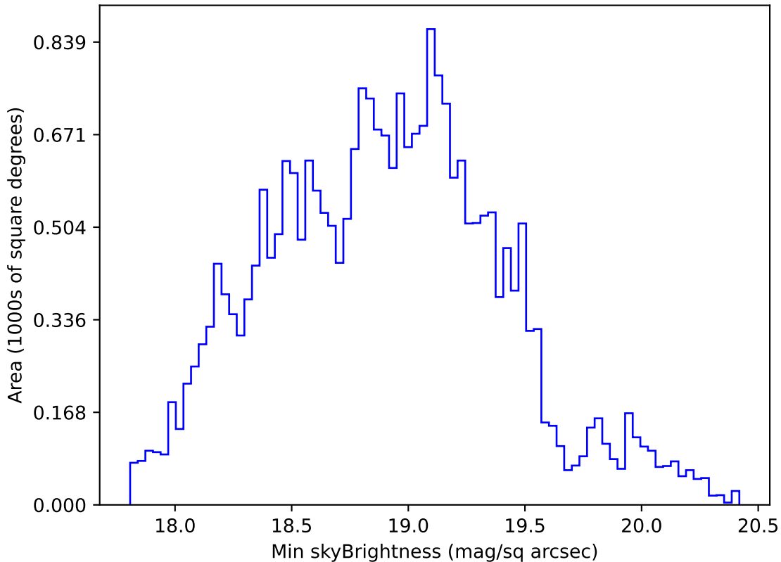
ddf_acor_sf10_lsf20_lsr10_v3.4_10yrs All sky r band: Min skyBrightness
